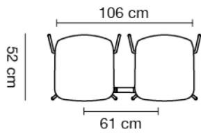
Pato 4 Leg Chair Seat coupling
