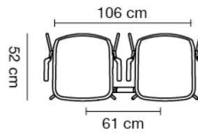
Pato 4 Leg Armchair Seat coupling
