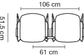
Pato Sledge Armchair Base coupling
