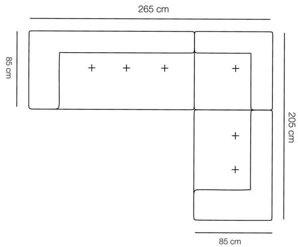
Model 450D, Configuration D MODEL 4514 (left) / 4513 / 4501 (right)
