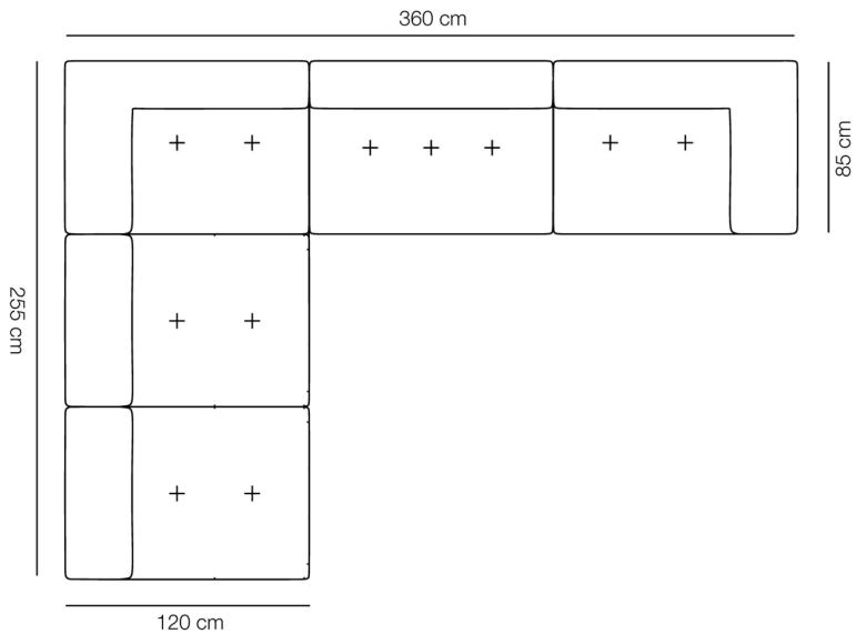
Model 450C, Configuration C MODEL 4503 / 4503 / 4501 (left) / 4502 / 4501 (right)
