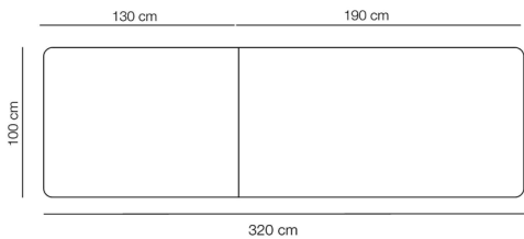
Model 665E, Configuration: E MODEL 6651 / 6651 + 1 pcs. 6650
