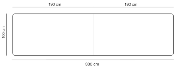
Model 665G, Configuration: G MODEL 6652 / 6654 / 6652 + 2. pcs. 6650
