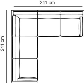
Model 209D, Configuration D 2047 L / 2099 / 2047 R
