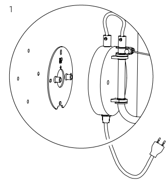
Installation wall 120
